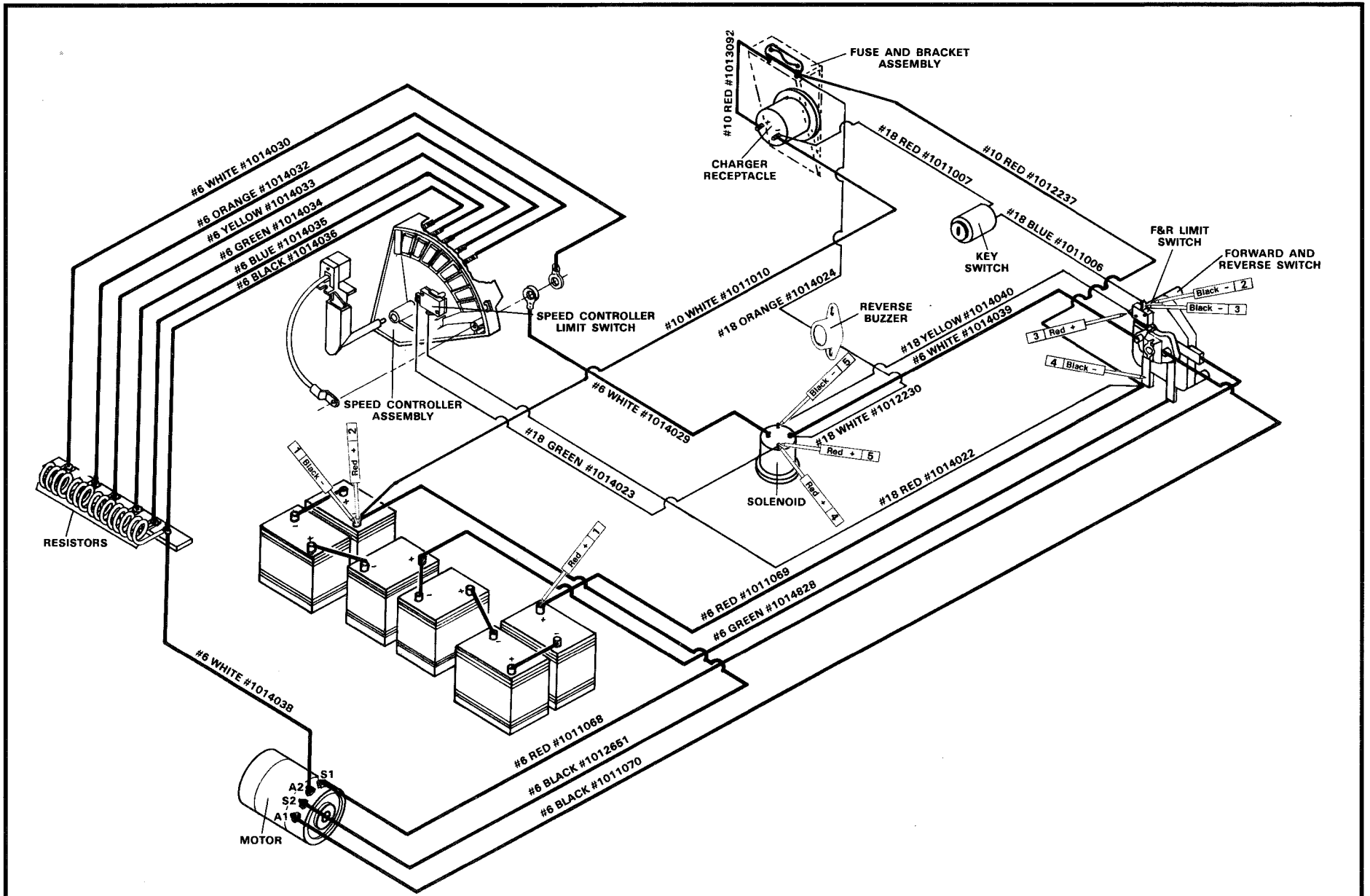
Figure 17-4 — Wiring Diagram with probes for control circuit testing
